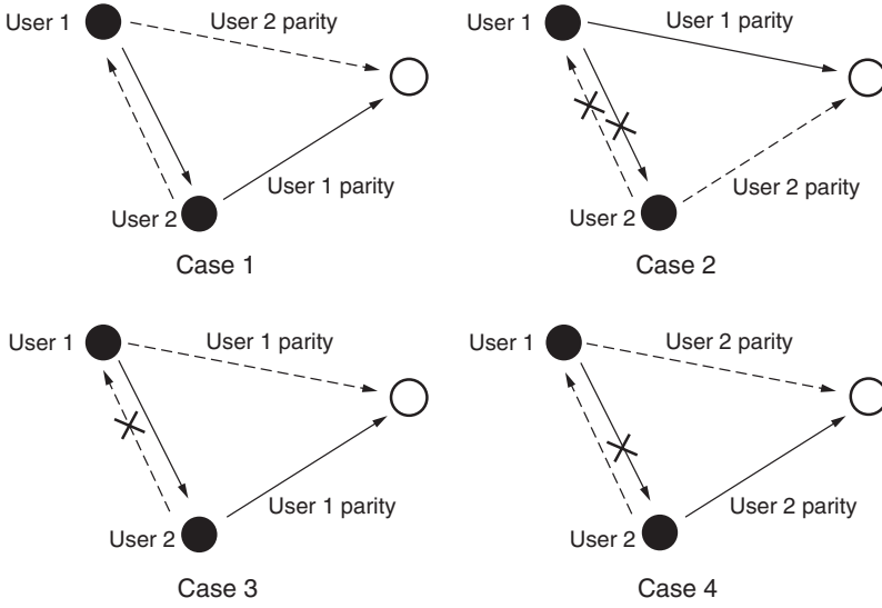
Figure 22.7 Four cases of messaging that can arise in two-user cooperative coding. Reproduced from Hunter and Nosratinia [2006] © IEEE.
