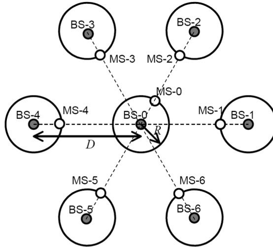
Figure 30.11 Cell structure.
