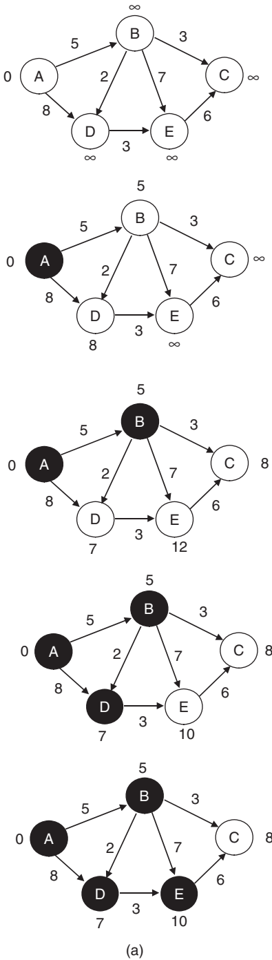
Figure 22.9 Dijkstra (a) and Bellman-Ford (b) algorithm.
