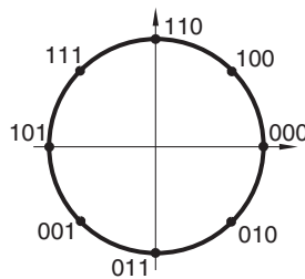
Figure 30.6 Grey-coded 8PSK.
