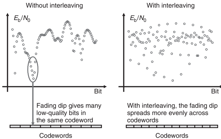
Figure 14.24 Effect of an interleaver.
