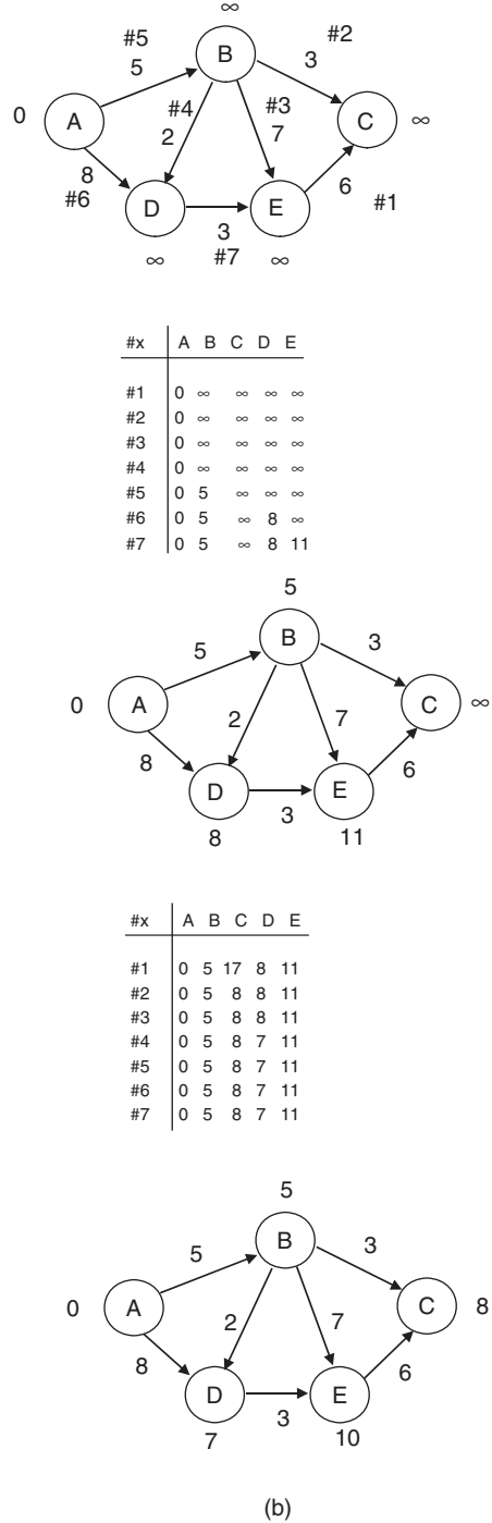
Figure 22.9 Dijkstra (a) and Bellman-Ford (b) algorithm.
