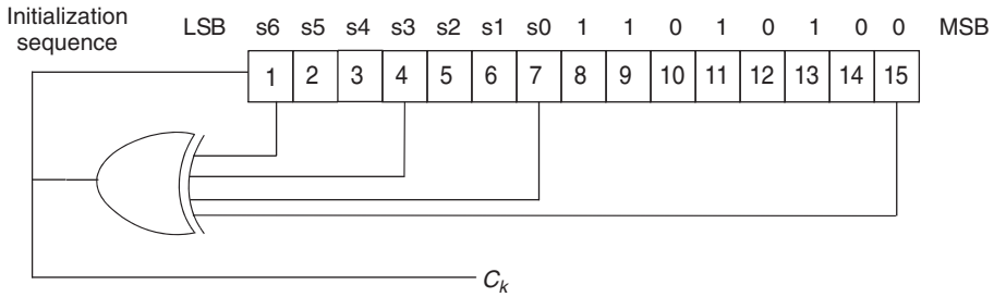
Figure 28.24 Shift register for generation of ranging code.
