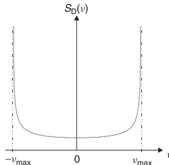
Figure 5.23 Classical Doppler spectrum.
