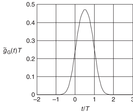
Figure 11.5 Shape of a Gaussian phase basis pulse with B_G T = 0.5 .
