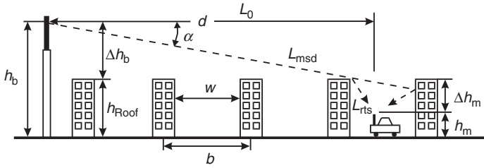
Figure 7.1 Parameters in the COST 231–Walfish–Ikegami model. Reproduced with permission from Damossio and Correia [1999] © European Union.
