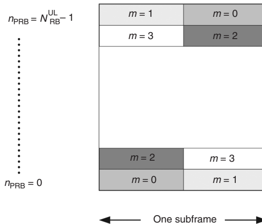
Figure 27.15 Resource assignment for the PUCCH.
