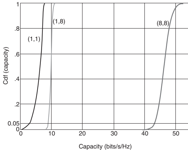
Figure 20.12 Cumulative distribution function of capacity for 1 × 1, 1 × 8, and the 8 × 8 optimum scheme.
