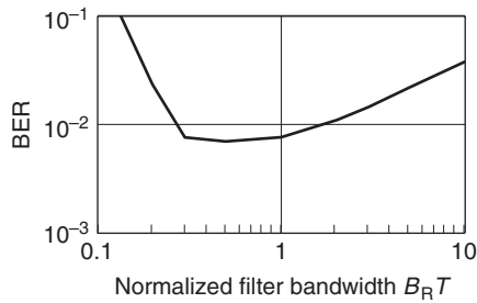
Figure 12.10 BER of filtered minimum shift keying with differential detection. The normalized rms delay spread is 0.1, and SNR = 12 dB.
