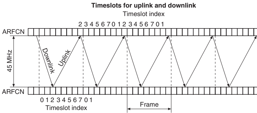
Figure 24.3 The alignment of timeslots in the uplinks and downlink. Adapted with permission from HP [1994] © Hewlett Packard.
