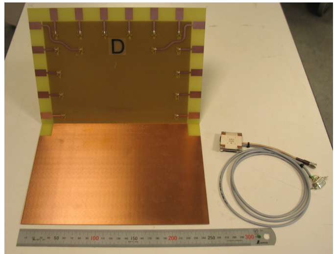
Fig. 6. The two arrays used at the MS’s. To the right the body-worn array is seen at the end of a cable with the four antenna elements at the corners. The size of the array is about 3 cm by 3 cm. To the left the laptop-like array is seen, consisting of two planes connected at an angle of about 110^\circ , with the plane on the table of size about 25 cm by 20 cm. Only four of the 16 elements along the edges are used, two at the top and one at each side of the ‘lid.’
