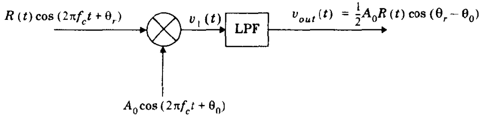
Figure 5.5 Block diagram of a product detector.
