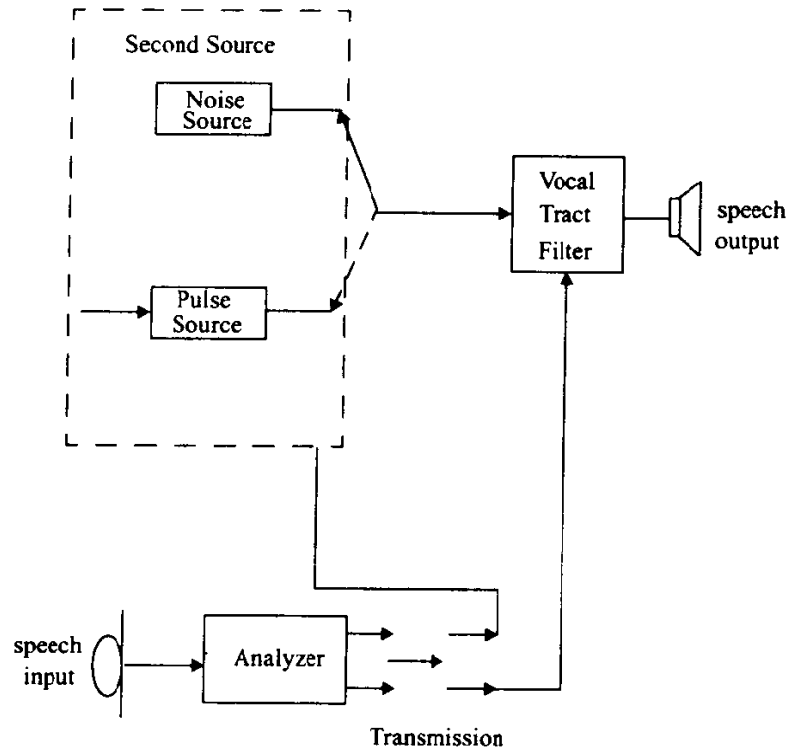
Figure 7.5 Speech generation model.
