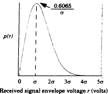
Figure 4.16 Rayleigh probability density function (pdf).
