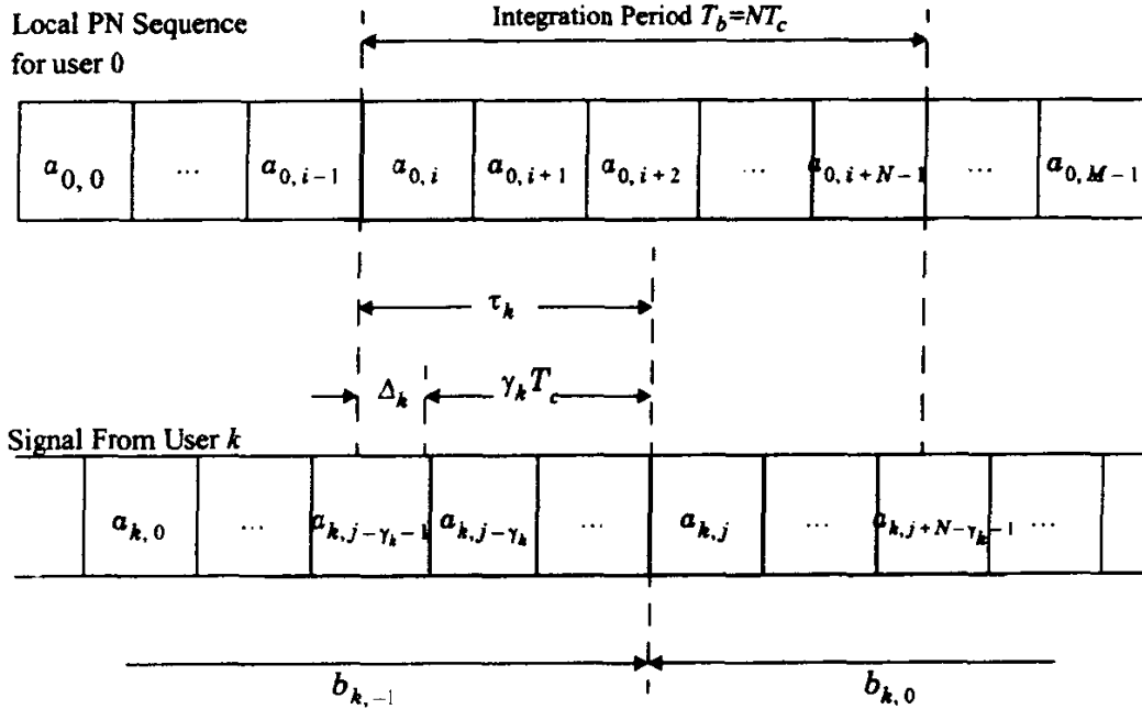
Figure C.2 Timing of the local PN sequence for user 0, a_0(t) , and the received signal from user k , s_k(t - \tau_k) .
