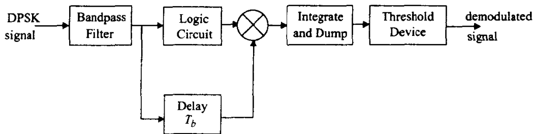
Figure 5.25 Block diagram of DPSK receiver.
