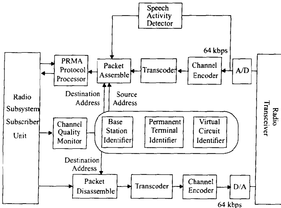
Figure 9.18 Cellular wireless interface unit [From [Goo90] © IEEE].
