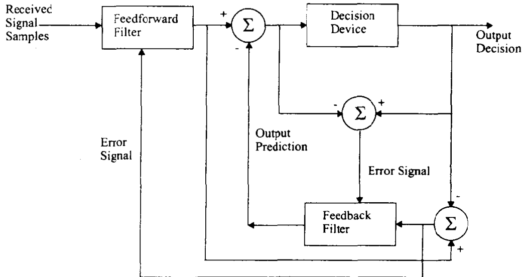
Figure 6.9 Predictive decision feedback equalizer.
