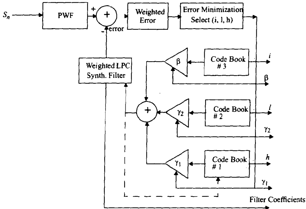
Figure 7.12 Block diagram of the USDC speech encoder.
