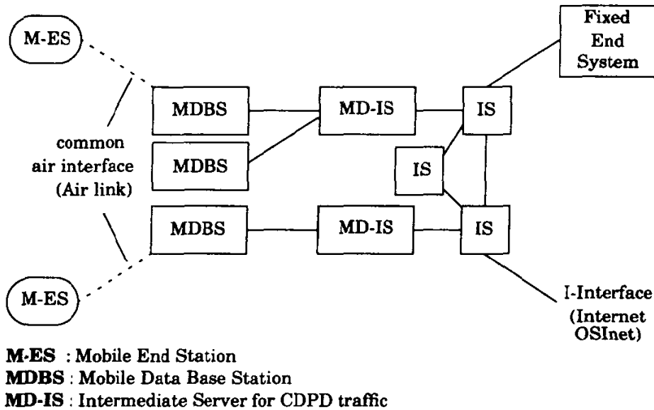
Figure 9.10 The CDPD network.
