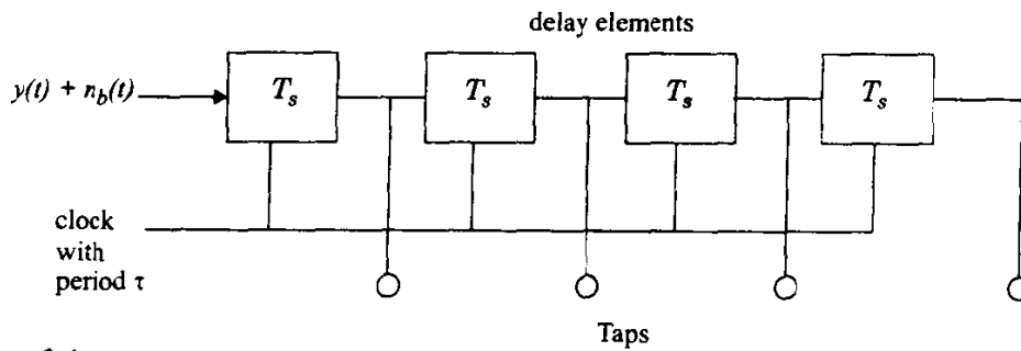
Figure 6.4 Basic linear transversal equalizer structure.
