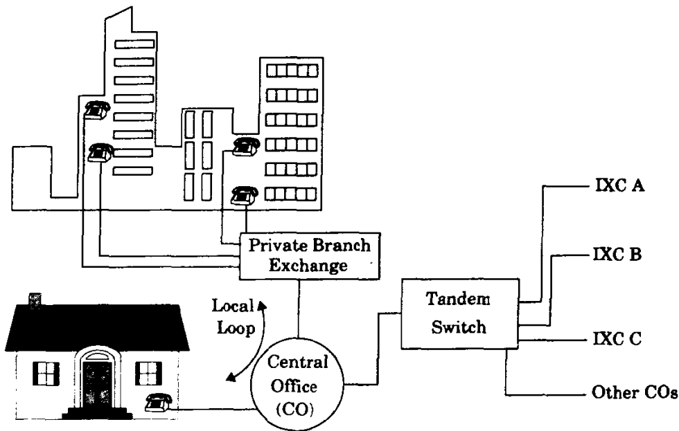
Figure 9.3 Local landline telephone network.
