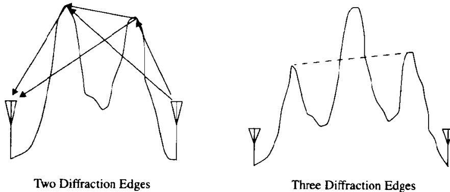
Figure 3.22 Illustration of multiple diffraction edges.
