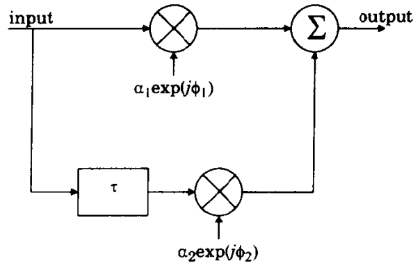
Figure 4.25 Two-ray Rayleigh fading model.
