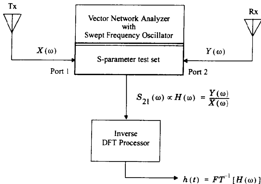
Figure 4.8 Frequency domain channel impulse response measurement system.
