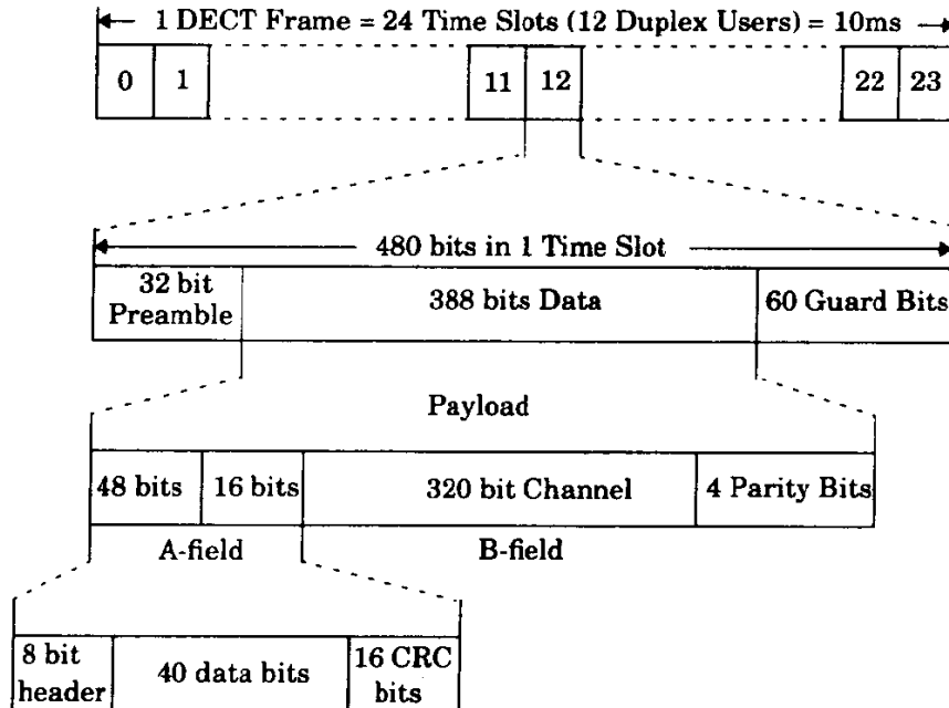
Figure 10.18 DECT TDMA frame structure.
