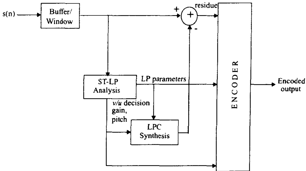
Figure 7.9 Block diagram of a RELP encoder.
