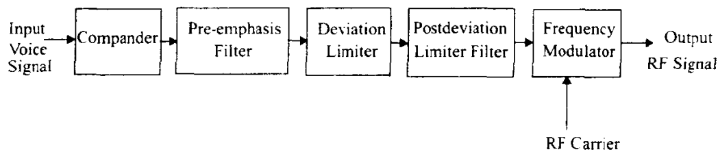
Figure 10.1 AMPS voice modulation process.
