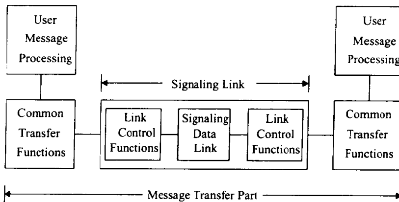
Figure 9.15 Functional diagram of message transfer part
