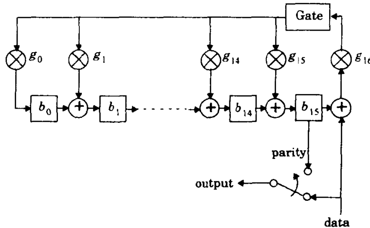
Figure 6.18 Reed-Solomon encoding circuit.
