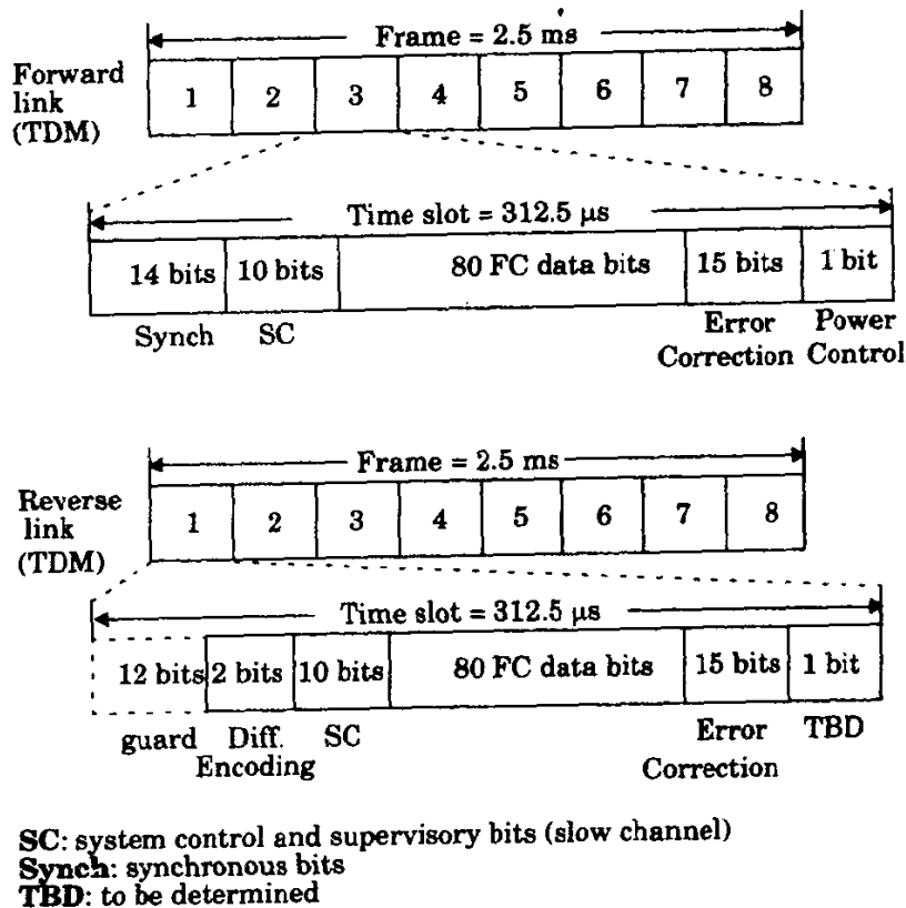
Figure 10.21 PACS Frame Structure
