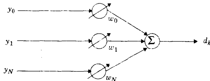
Figure P6.1: Multiple input adaptive linear combiner.
