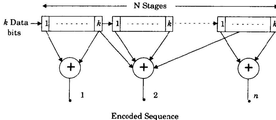
Figure 6.19 General block diagram of convolutional encoder.
