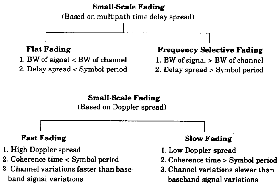
Figure 4.11 Types of small-scale fading.
