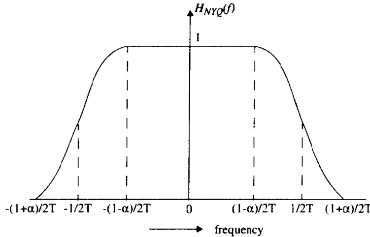
Figure 5.16 Transfer function of a Nyquist pulse-shaping filter.
