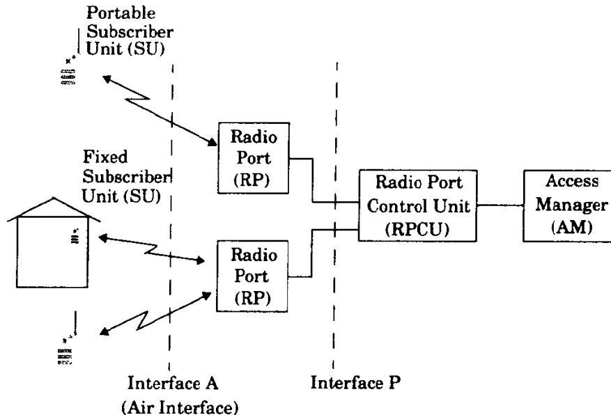
Figure 10.20 PACS system architecture.
