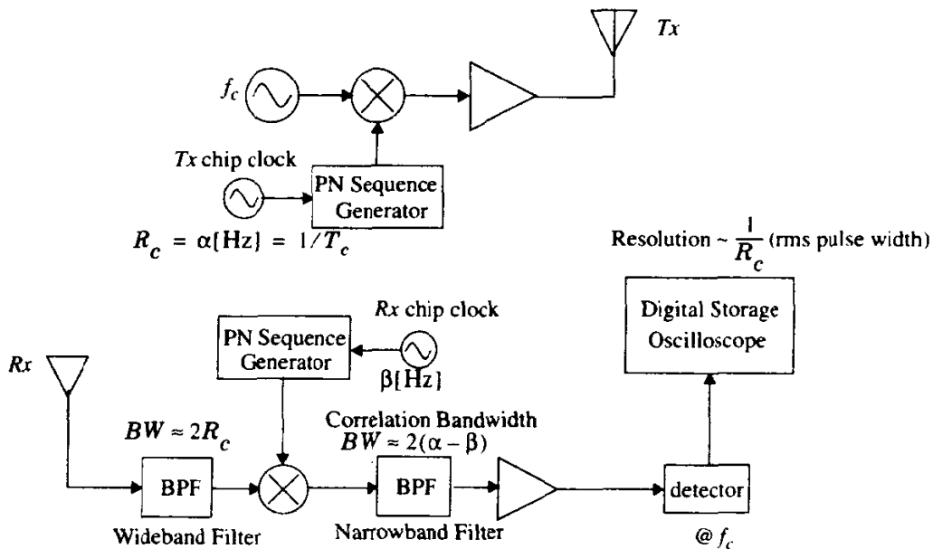
Figure 4.7 Spread spectrum channel impulse response measurement system.
