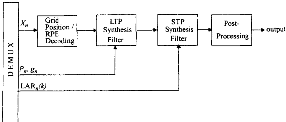
Figure 7.11 Block diagram of GSM speech decoder.
