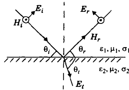
(a) E-field in the plane of incidence
