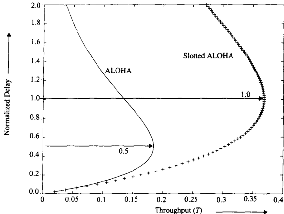
Figure 8.10 Trade-off between throughput and delay for ALOHA and slotted ALOHA packet radio protocols.
