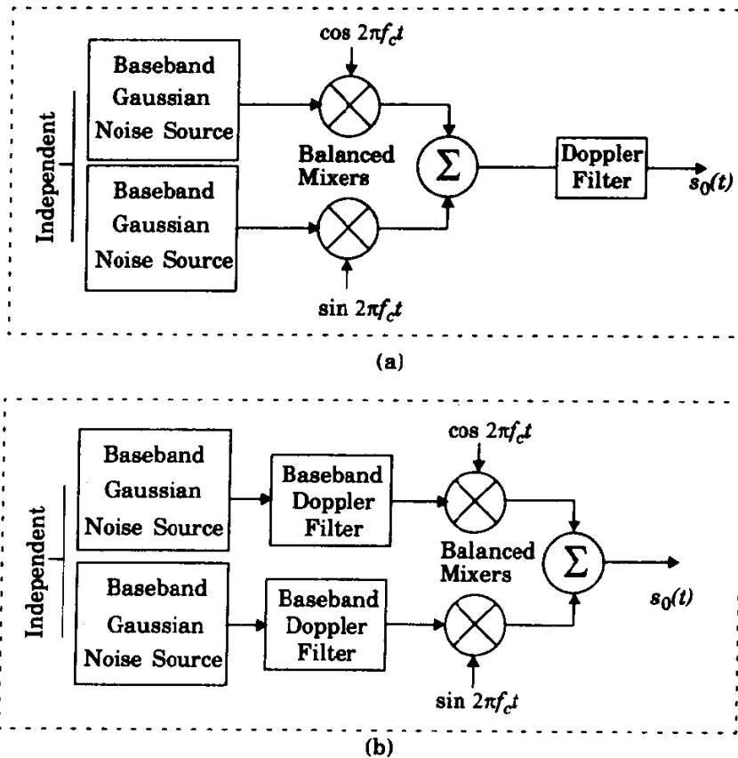
Figure 4.22 Simulator using quadrature amplitude modulation with (a) RF Doppler filter and (b) baseband Doppler filter.
