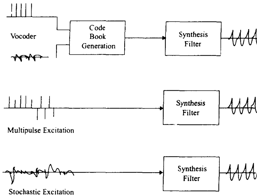
Figure 7.7 LPC excitation methods.
