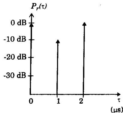
Figure P4.18. Power delay profile.
