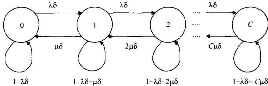
Figure A.1 The transition probabilities represented as a Markov chain state diagram for Erlang B.
