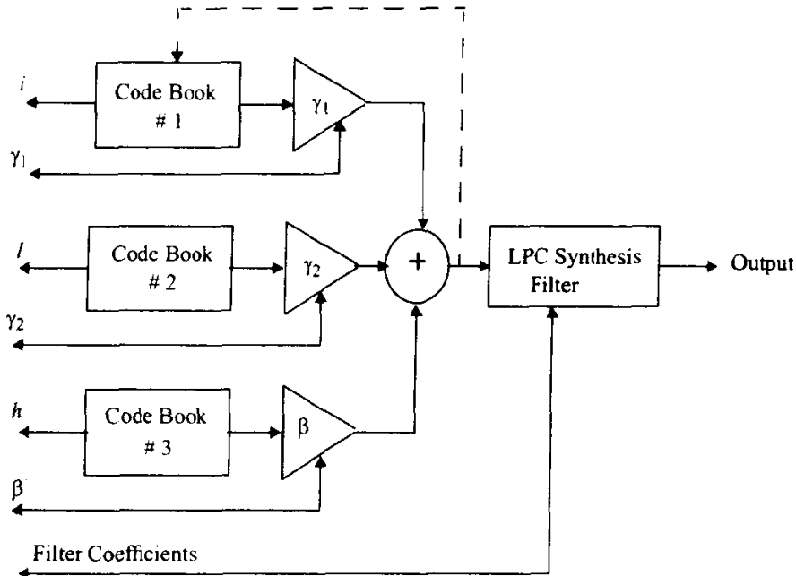
Figure 7.13 Block diagram of the USDC speech decoder.
