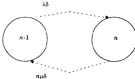
Figure A.2 A trunked LCC system at steady state with n number of channels in use.
