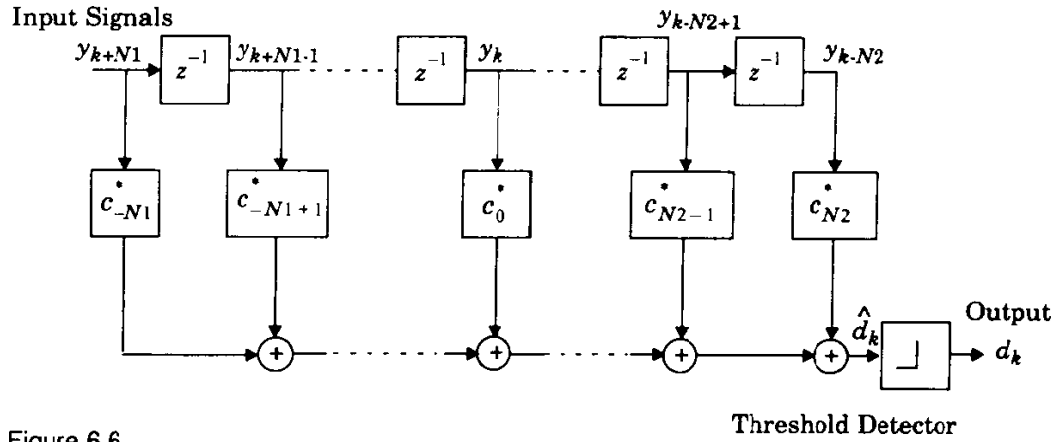
Figure 6.6 Structure of a linear transversal equalizer.
