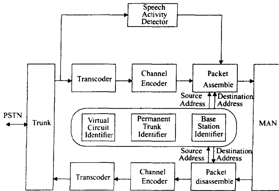
Figure 9.17 Cellular trunk interface unit [From [Goo90] © IEEE].
