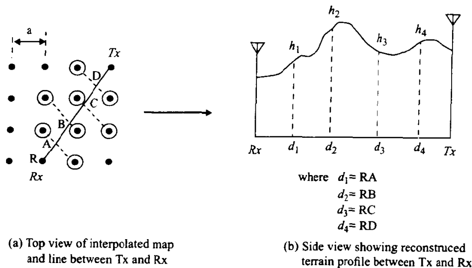
Figure 3.20 Illustration of terrain profile reconstruction using diagonal interpolation.
