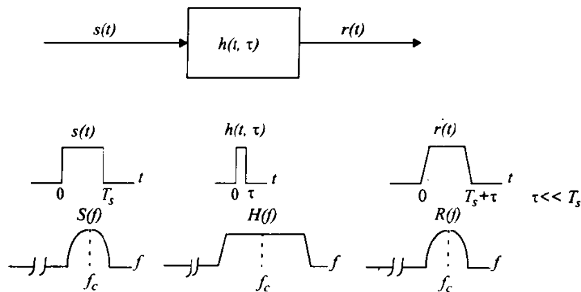
Figure 4.12 Flat fading channel characteristics.
