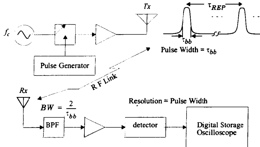
Figure 4.6 Direct RF channel impulse response measurement system.
