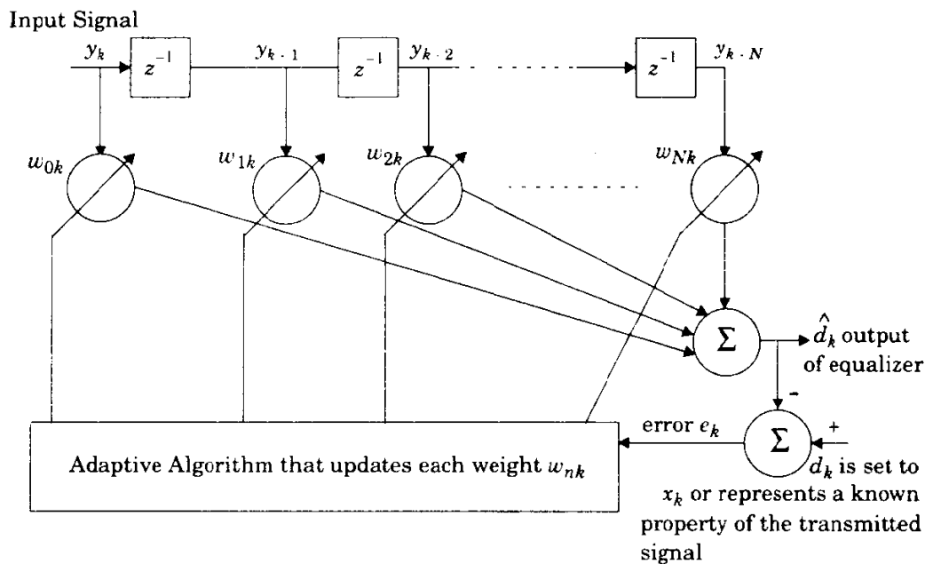
Figure 6.2 A basic linear equalizer during training.
