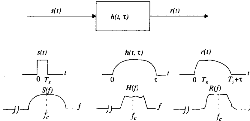
Figure 4.13 Frequency selective fading channel characteristics.
