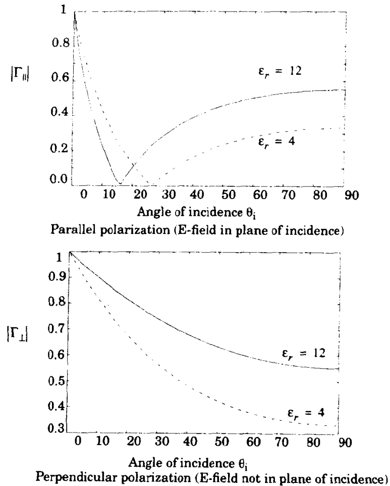
Figure 3.6 Magnitude of reflection coefficients as a function of angle of incidence for \epsilon_r = 4 , \epsilon_r = 12 , using geometry in Figure 3.4.
