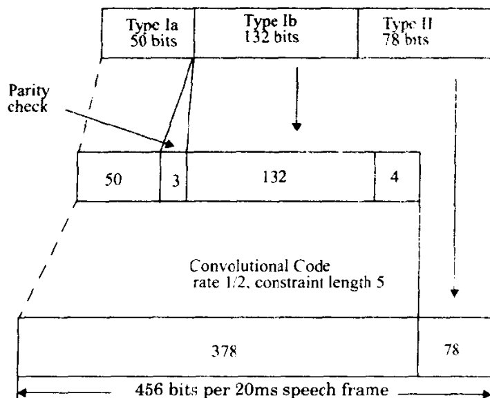
Figure 10.12 Error protection for speech signals in GSM.
