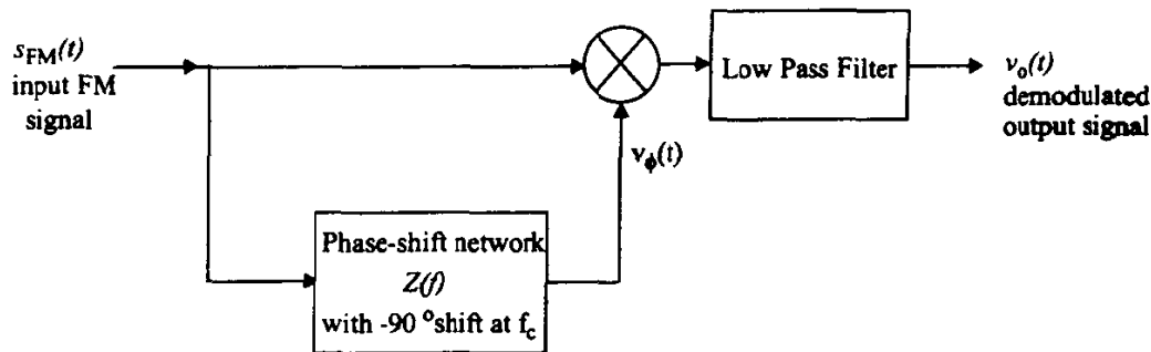
Figure 5.12 Block diagram of a quadrature detector.
