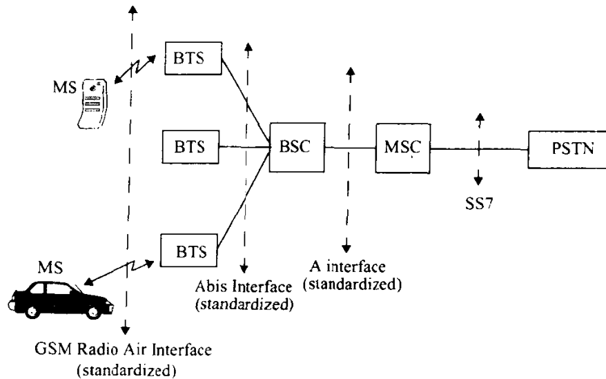
Figure 10.6 The various interfaces used in GSM.
