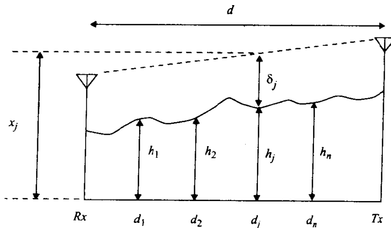
Figure 3.21 Illustration of line-of-sight (LOS) decision making process.
