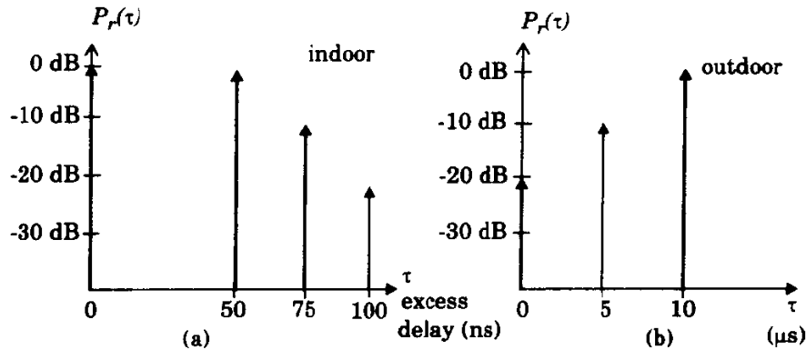
Figure P4.2: Two channel responses for Problem 4.2
