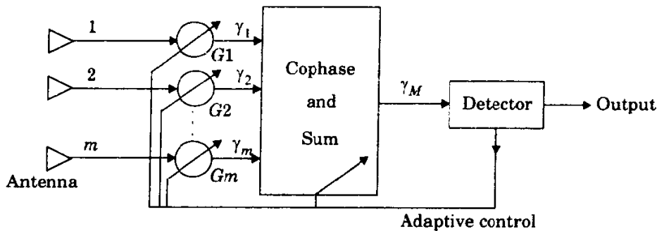
Figure 6.14 Maximal ratio combiner.
