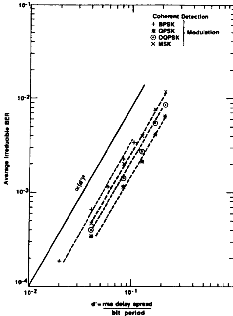
Figure 5.55 The same set of curves as plotted in Figure 5.54 plotted as a function of rms delay spread normalized by bit period [From [Chu87] © IEEE].
