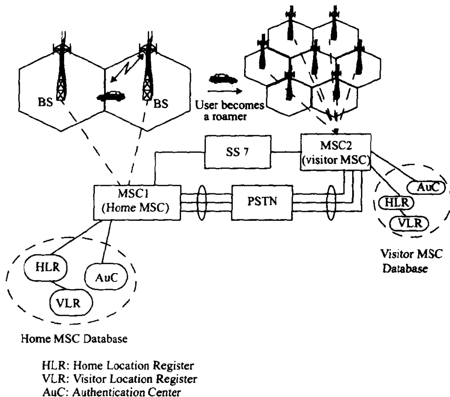
Figure 9.5 Block diagram of a cellular radio network.
