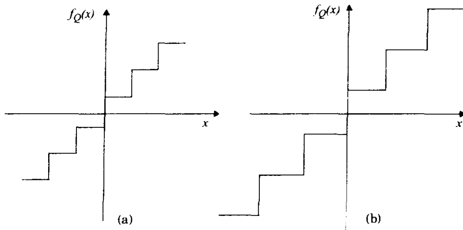
Figure 7.2 Adaptive quantizer characteristics (a) when the input signal has a low amplitude swing and (b) when the input signal has a large amplitude swing.
