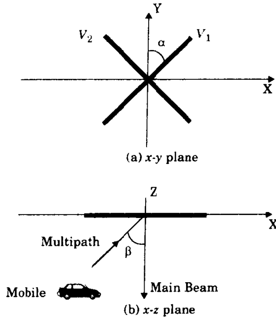
Figure 6.15 Theoretical Model for base station polarization diversity based on [Koz85].
