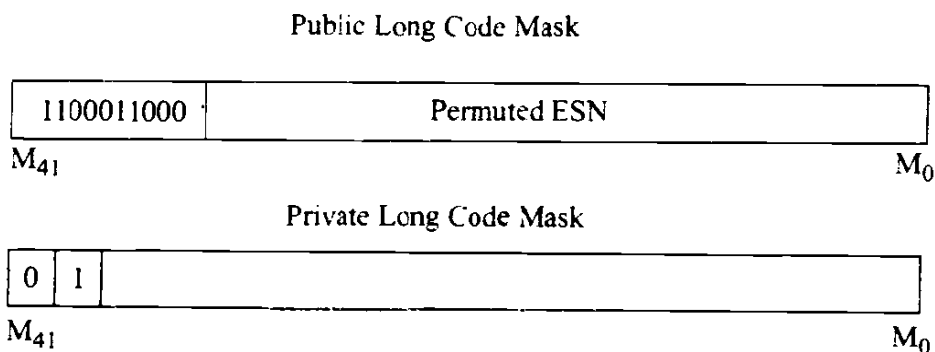
Figure 10.15 Long code mask format for IS-95.
